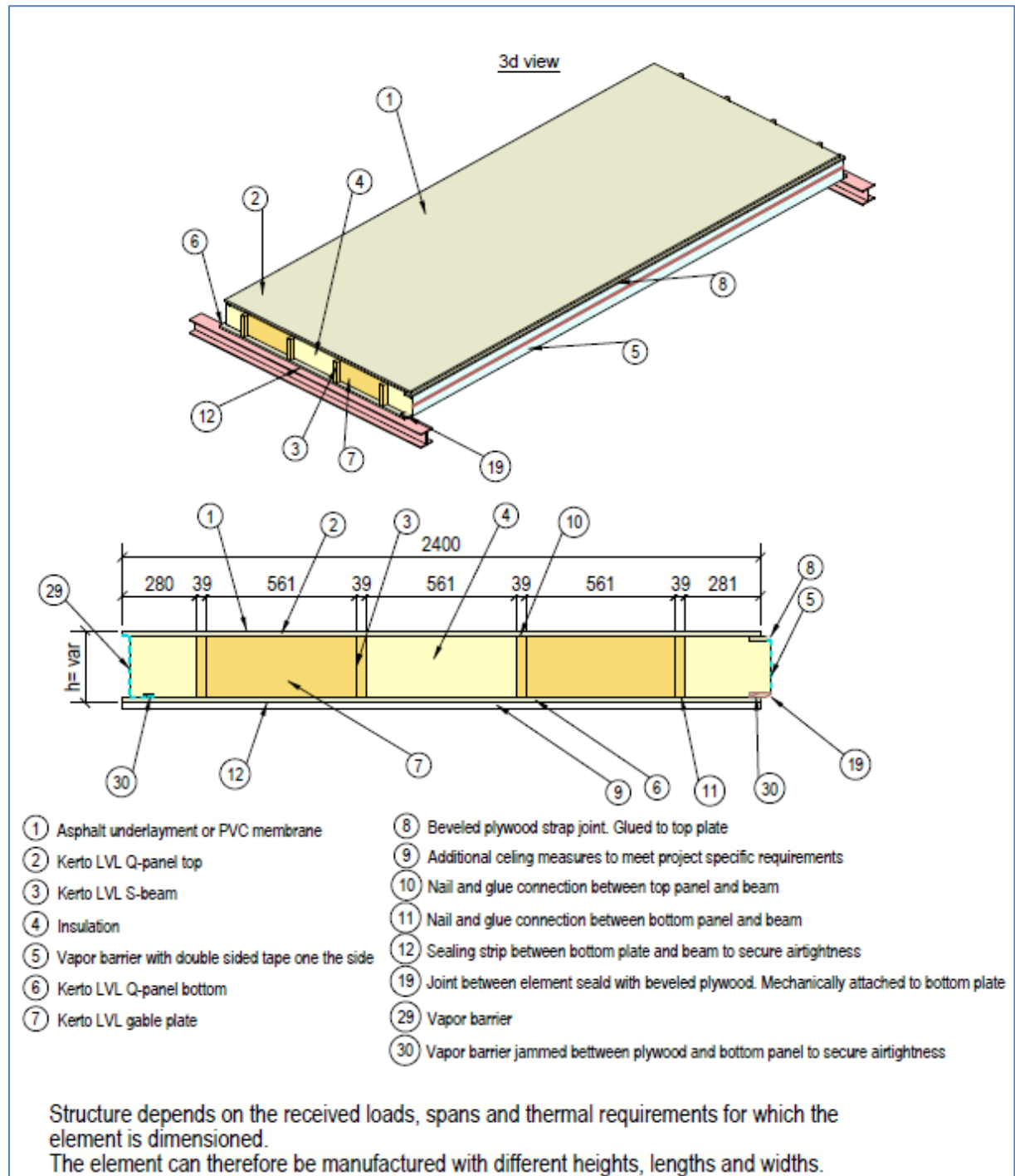
Figure1-1: 3D view and cross section of Lett-Tak wood (LTW) roof element with a glued Kerto LVL Q panel at the bottom.
