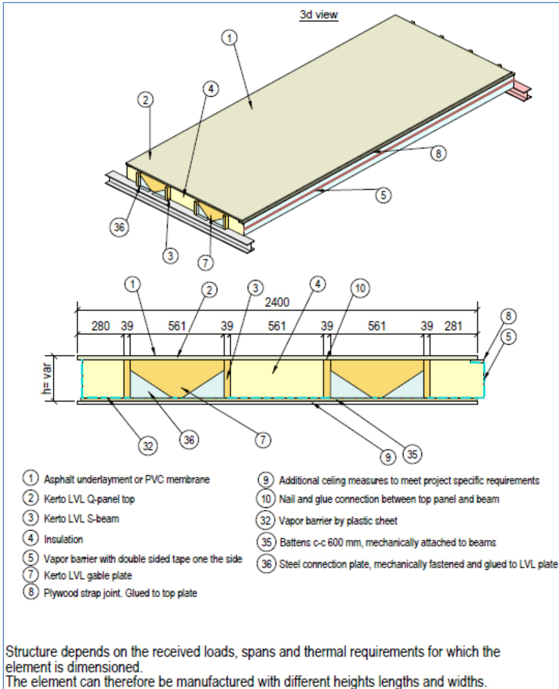
Figure1-3: 3D view and cross section of Lett-Tak wood (LTW) roof element without a load bearing Kerto LVL Q panels at the bottom.
