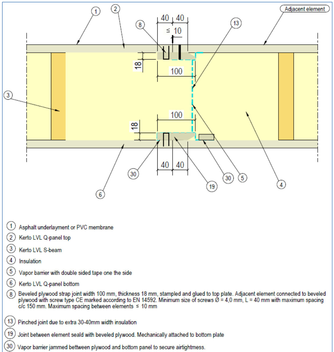
Figure1-6: Principal drawing of a joint between Lett-Tak wood (LTW) roof elements.
