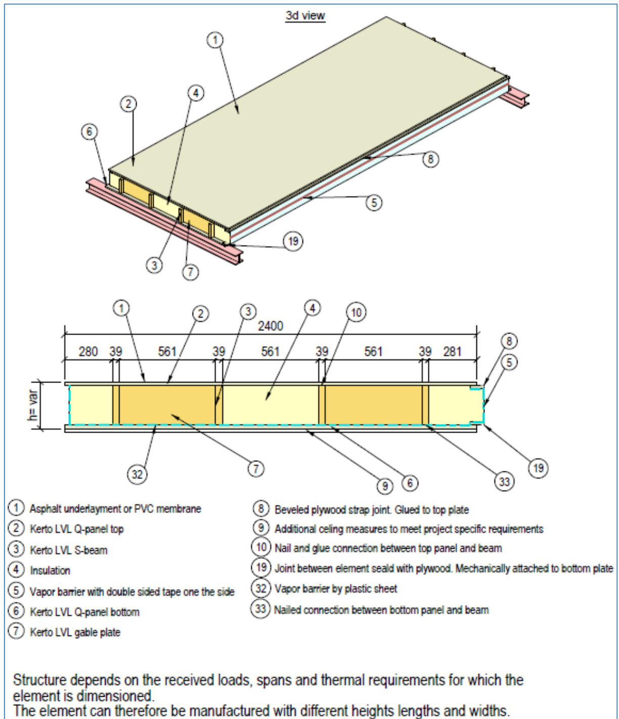
Figure1-2: 3D view and cross section of Lett-Tak wood (LTW) roof element with a nailed Kerto LVL Q panel at the bottom and plastic vapour barrier membrane.
